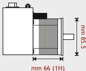
mm 66 (1H) Holding Torque: 360 Ncm
