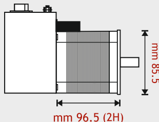
mm 96.5 (2H) Holding Torque: 700 Ncm
